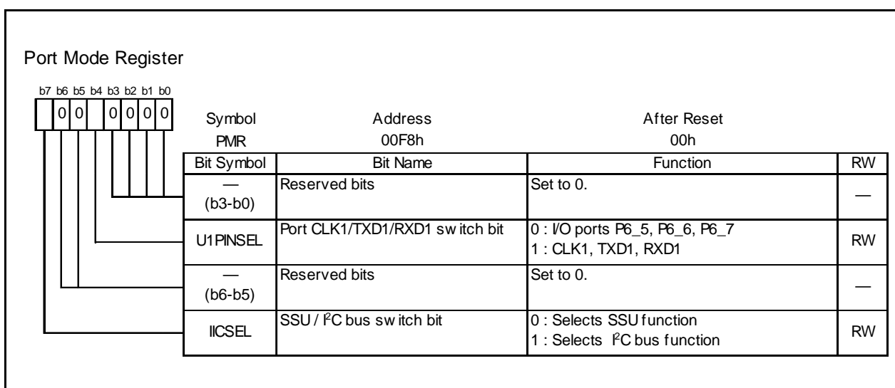
Figure 16.9 PMR Register
