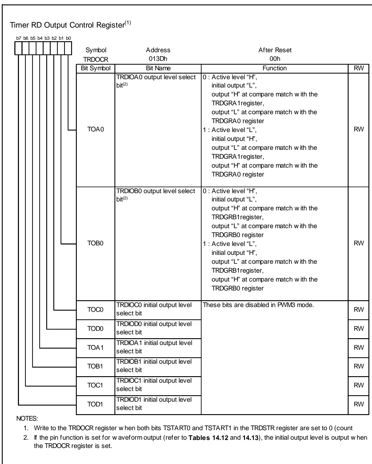
Figure 14.101 TRDOCR Register in PWM3 Mode
