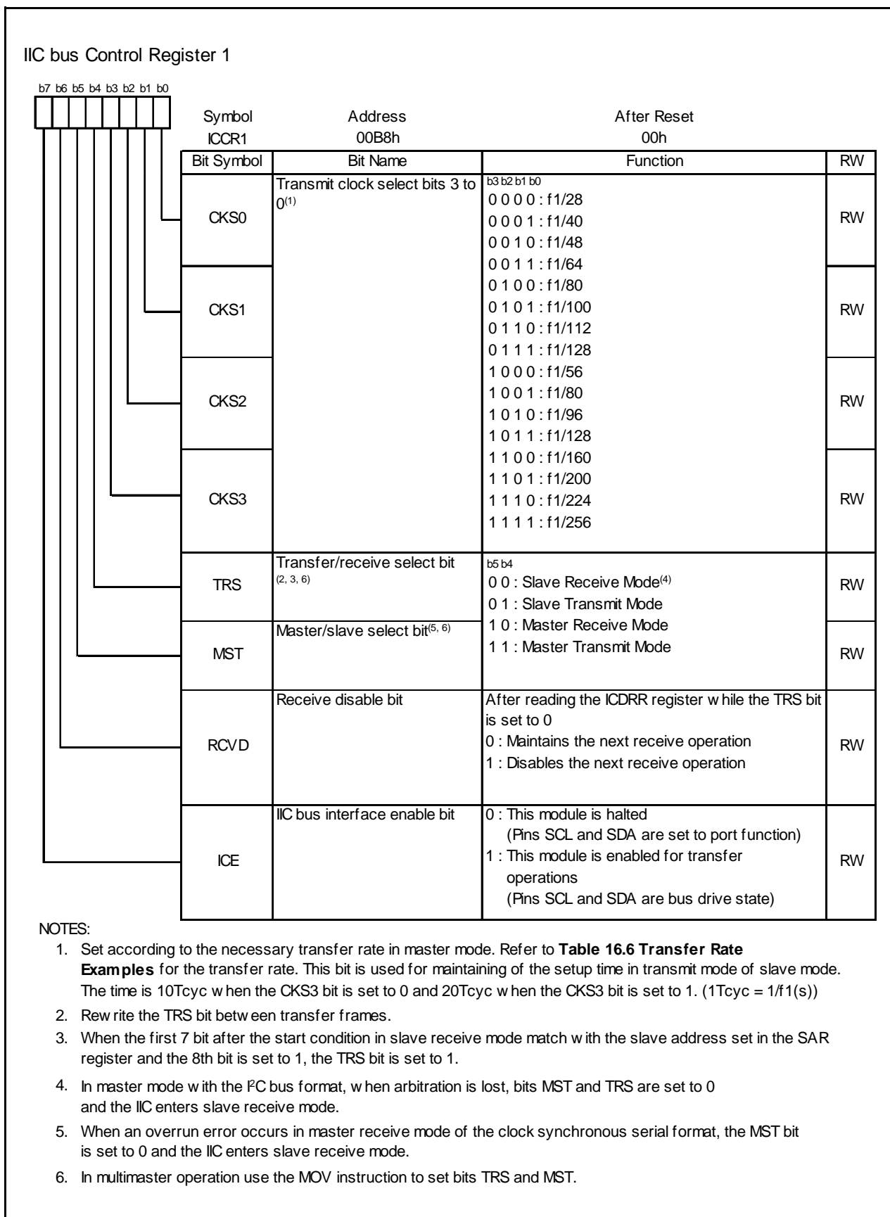
Figure 16.24 ICCR1 Register
