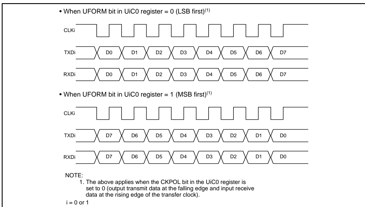
Figure 15.9 Transfer Format
